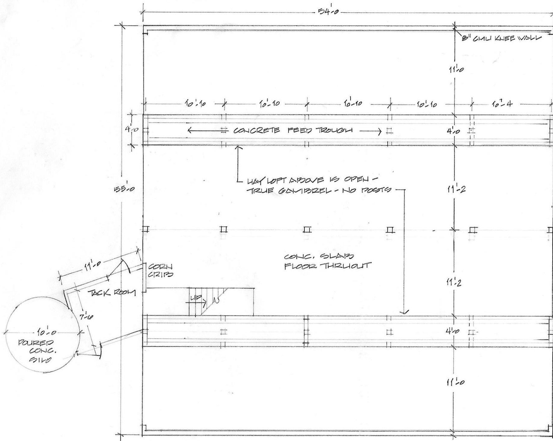
HOMER REEVES DAIRY BARN SCALE \frac{1}{8}'' = 1'-0'' FIRST FLOOR PLAN
