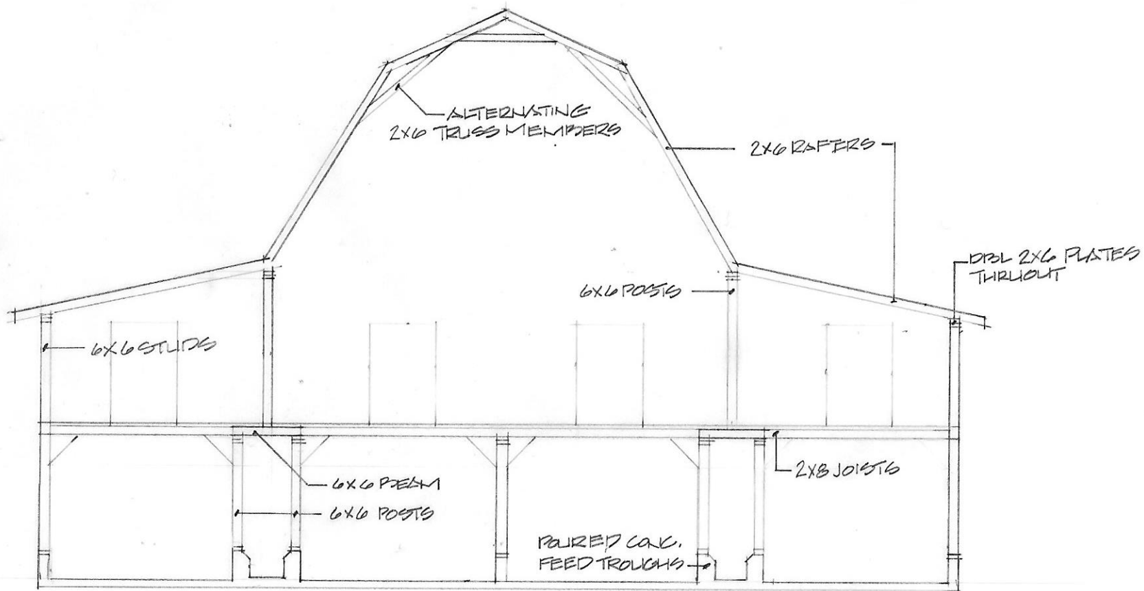
HOMER REEVES DAIRY BARN FRAMING SECTION SCALE \frac{1}{8}'' = 1'-0''
