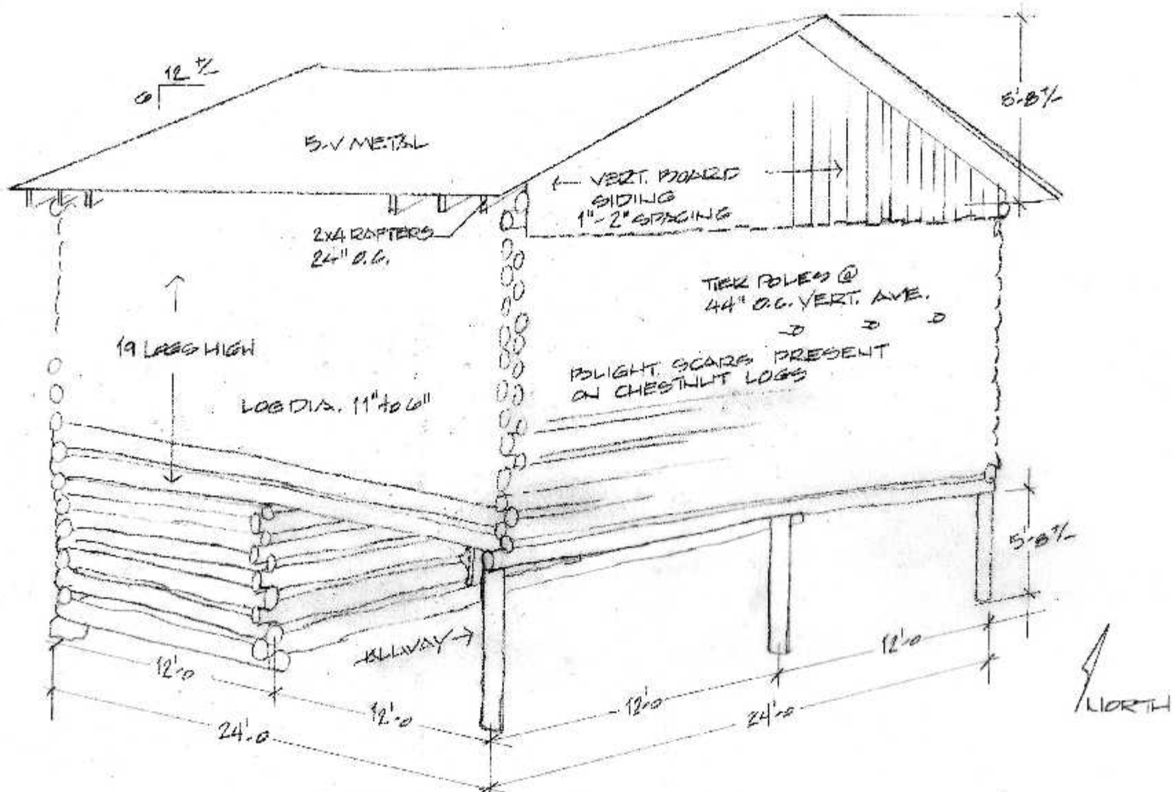
FURMAN WILLET LOG LIVESTOCK BARN 3/4 VIEW NO SCALE
