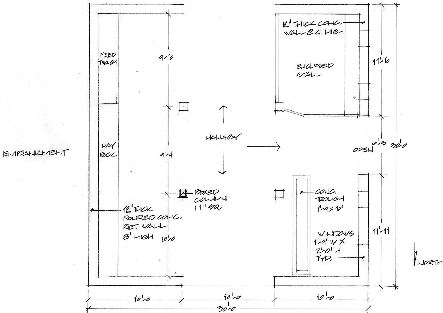
PANIE LUSK LIVESTOCK BARN GROUND FLOOR PLAN \frac{3}{16}'' = 1'-0''
