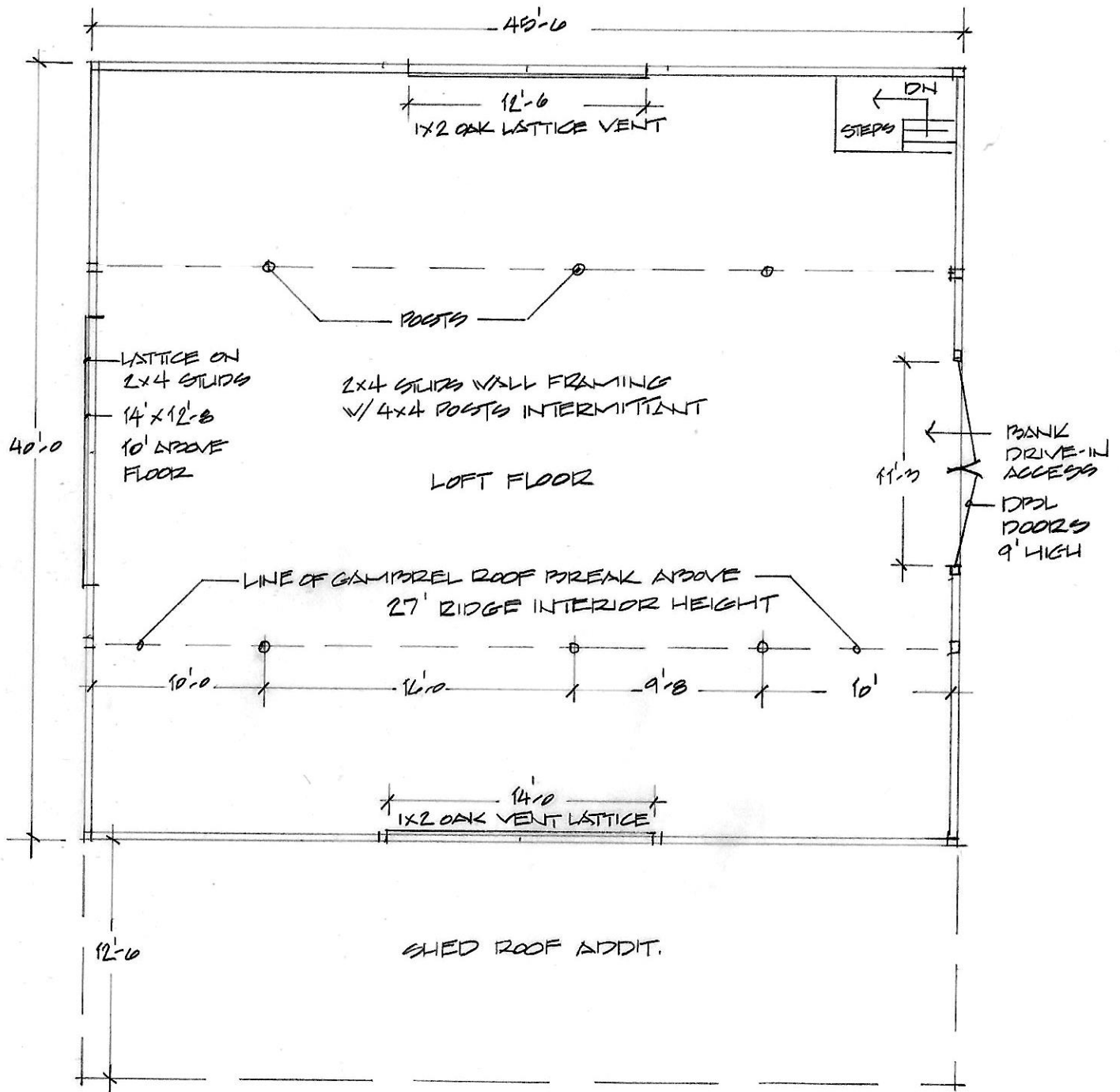
METCALF-PRICE LIVESTOCK BARN LOFT FLOOR - PLAN SCALE 1/8" = 1'-0"
