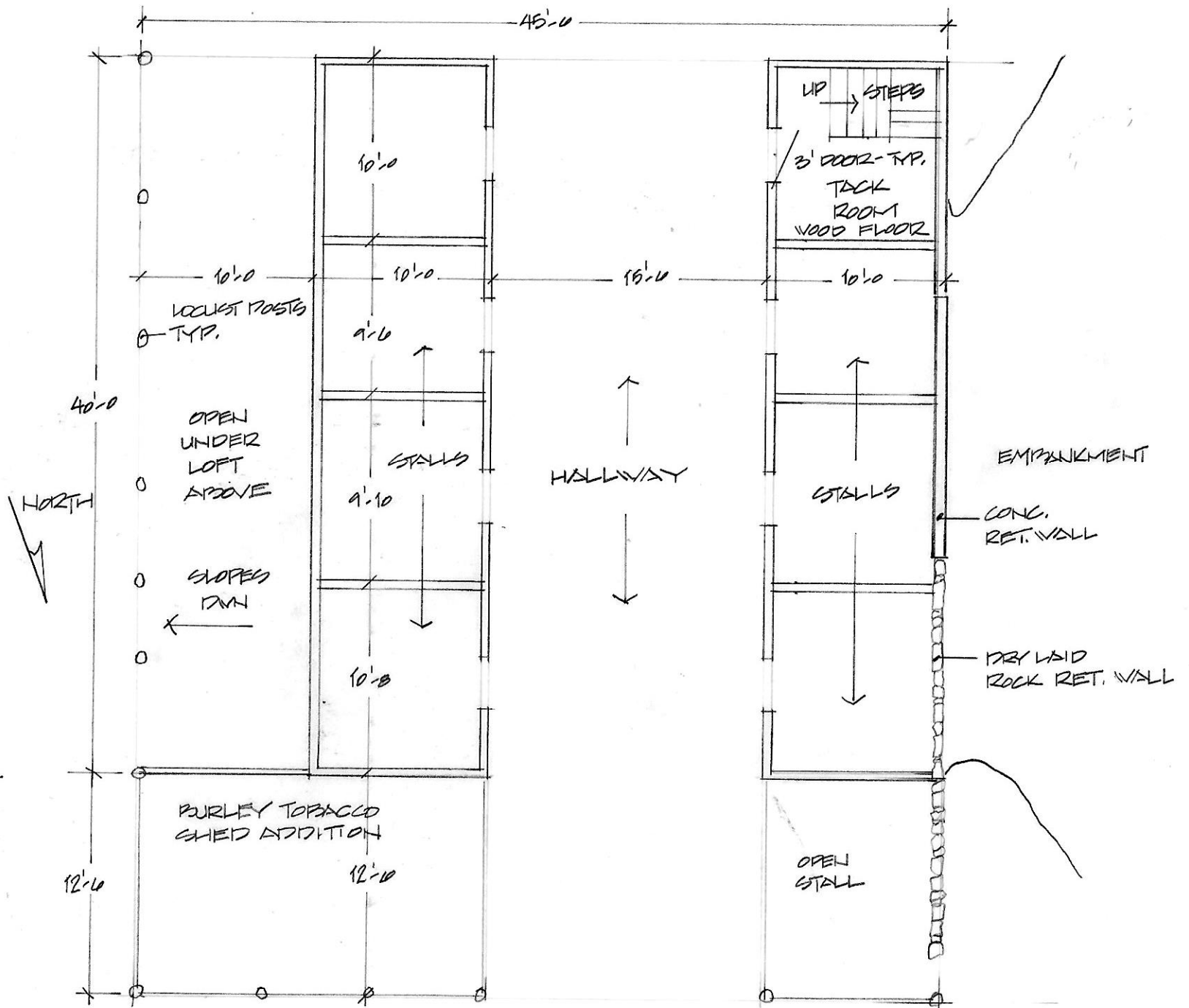
METCALF-PRICE LIVESTOCK BARN GROUND FLOOR - PLAN SCALE 1/8" = 1'-0"
