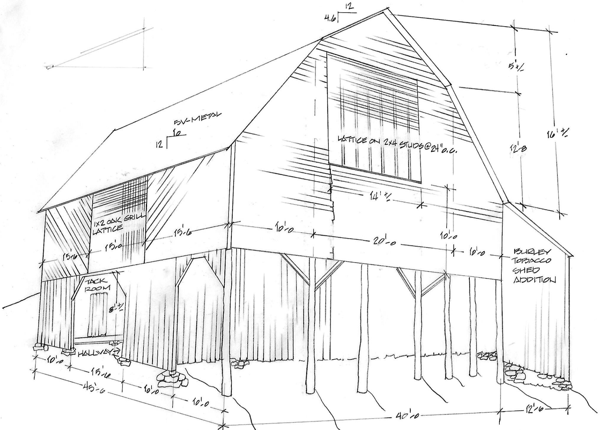
METCALF-PRICE LIVESTOCK BARN 3-QTR VIEW NO SCALE
