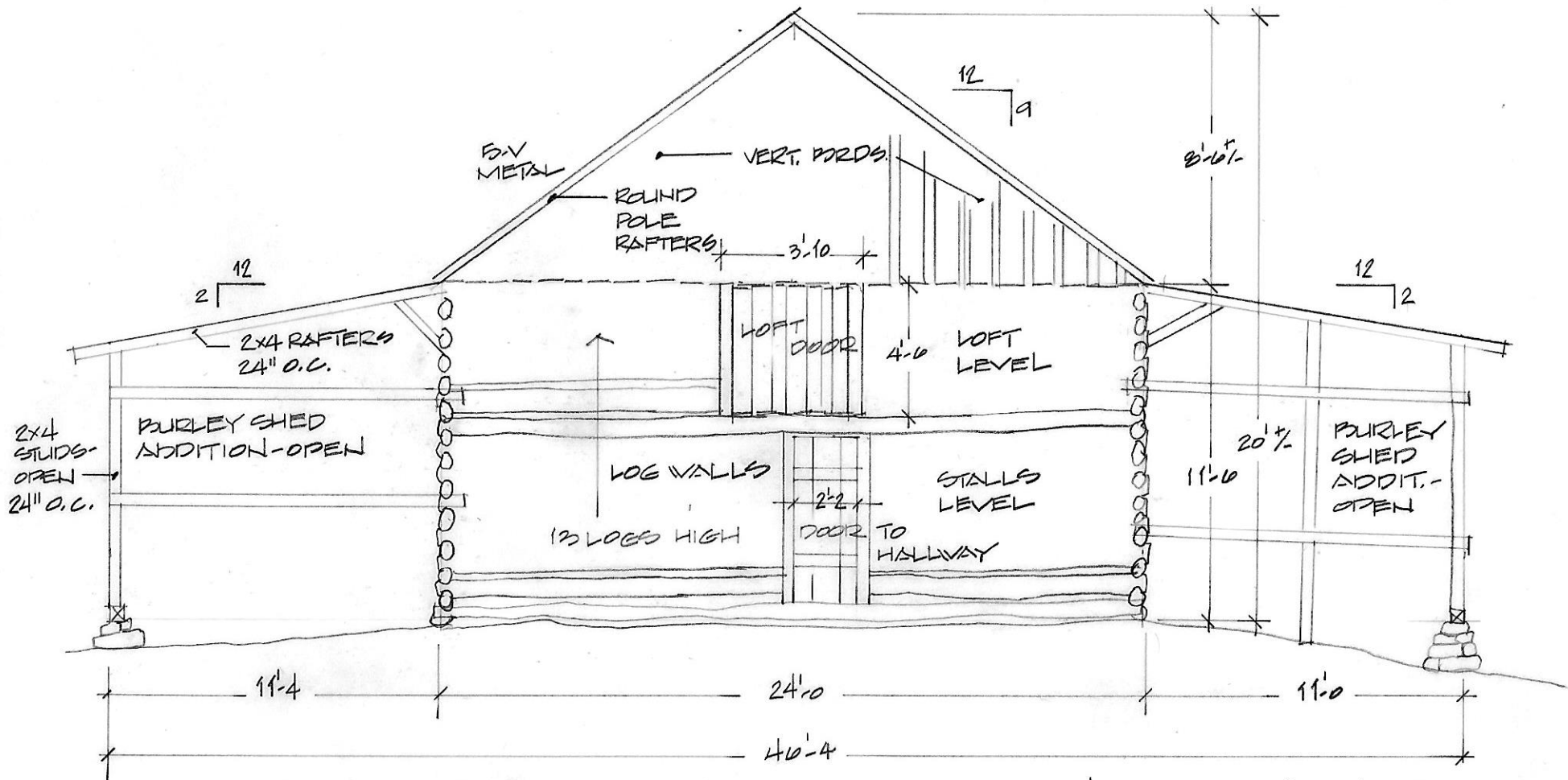
HENRY DAVIS LIVESTOCK BARN NORTH ELEVATION
