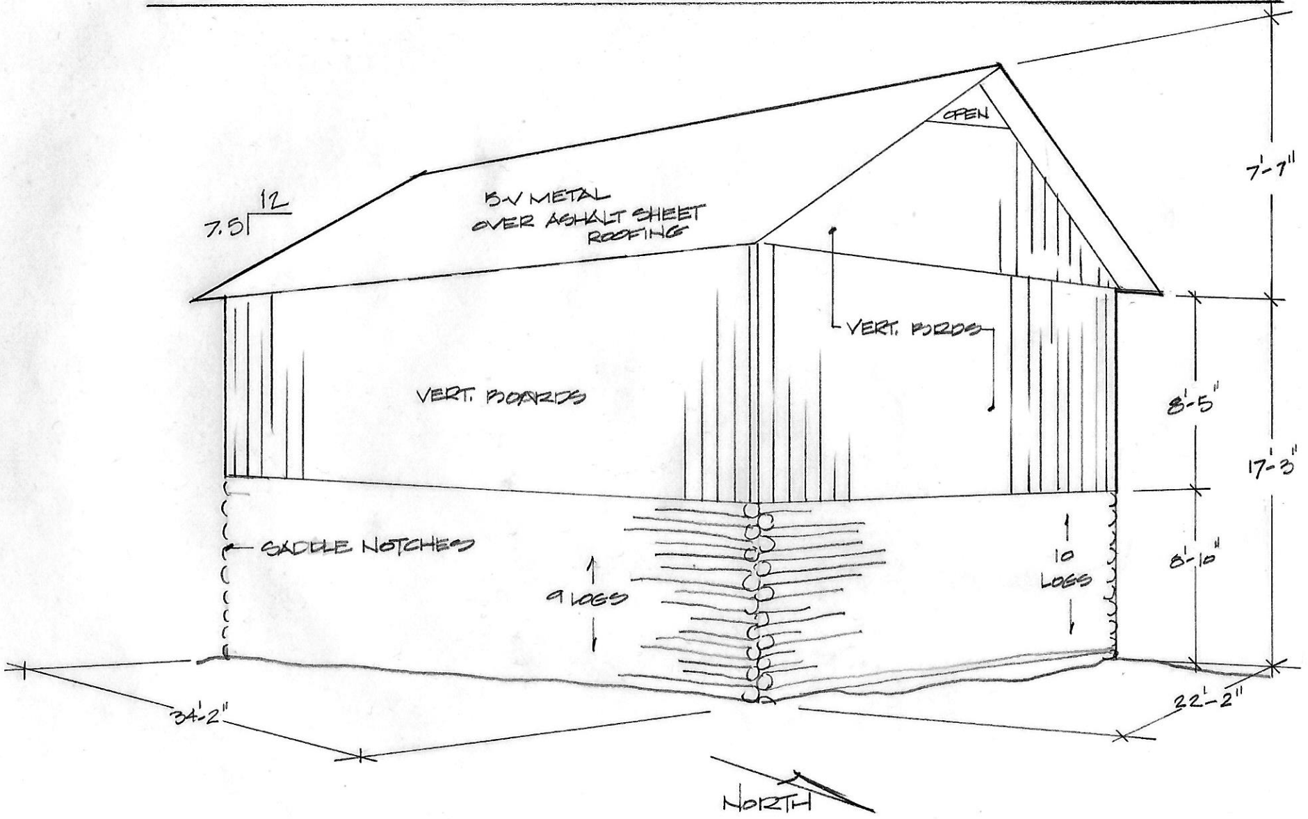
3/4 VIEW FROM NORTHEAST NO SCALE
