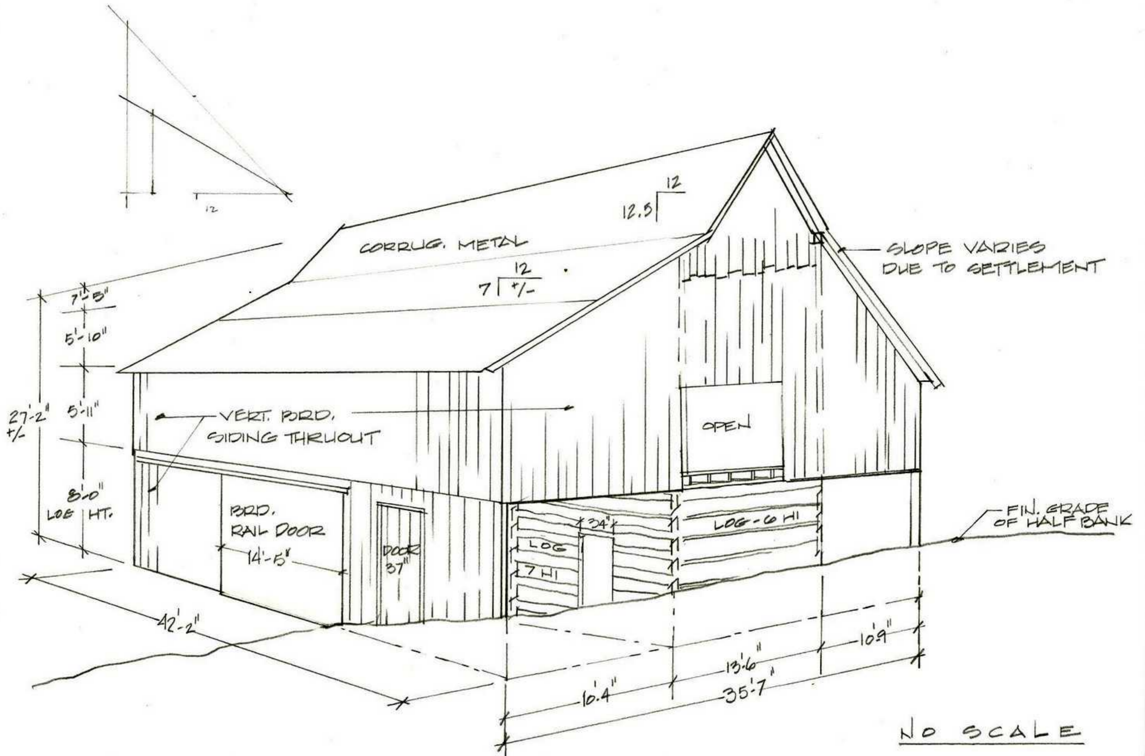
3/4 PERSPECTIVE VIEW W/N LOOKING SOUTHEAST
