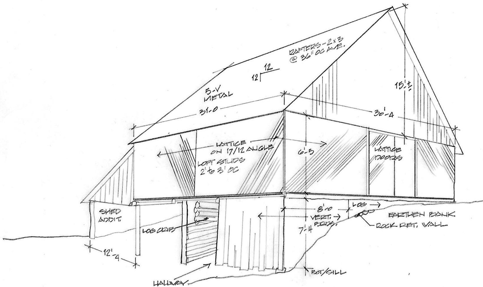
3/4 QTR VIEW NO SCALE W. W. WHITE LIVESTOCK BARN
