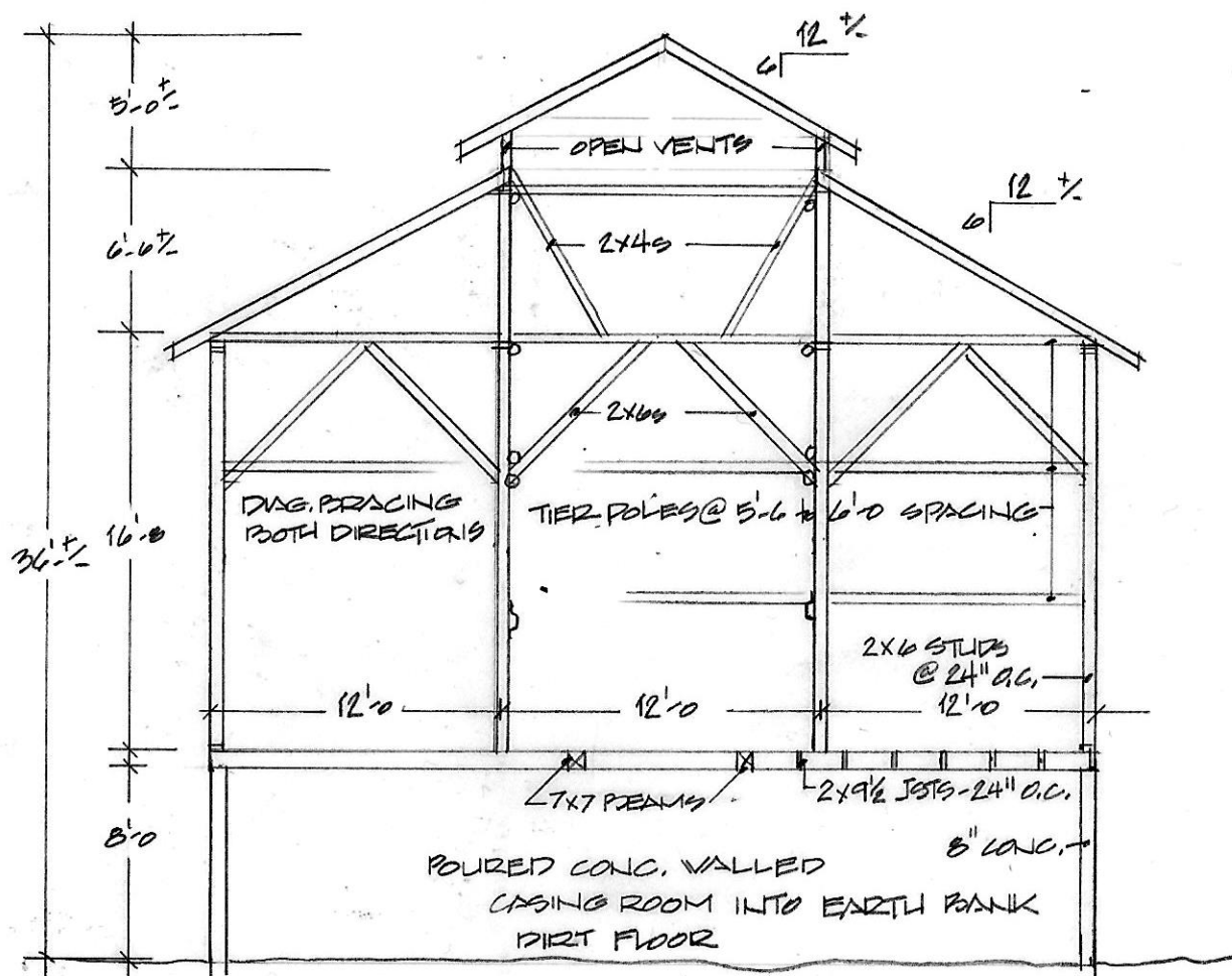
WOODS AMMONS PURLEY BARN #1 SECTION \frac{1}{8}'' = 1'-0''
