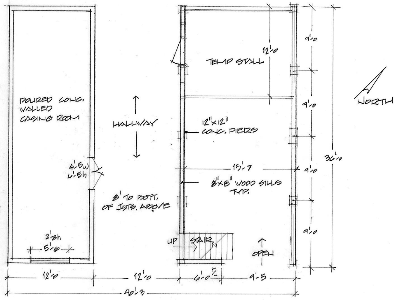
WOODS AMMONS BURLEY BARN #1 GROUND FLOOR PLAN 1/8" = 1'-10"
