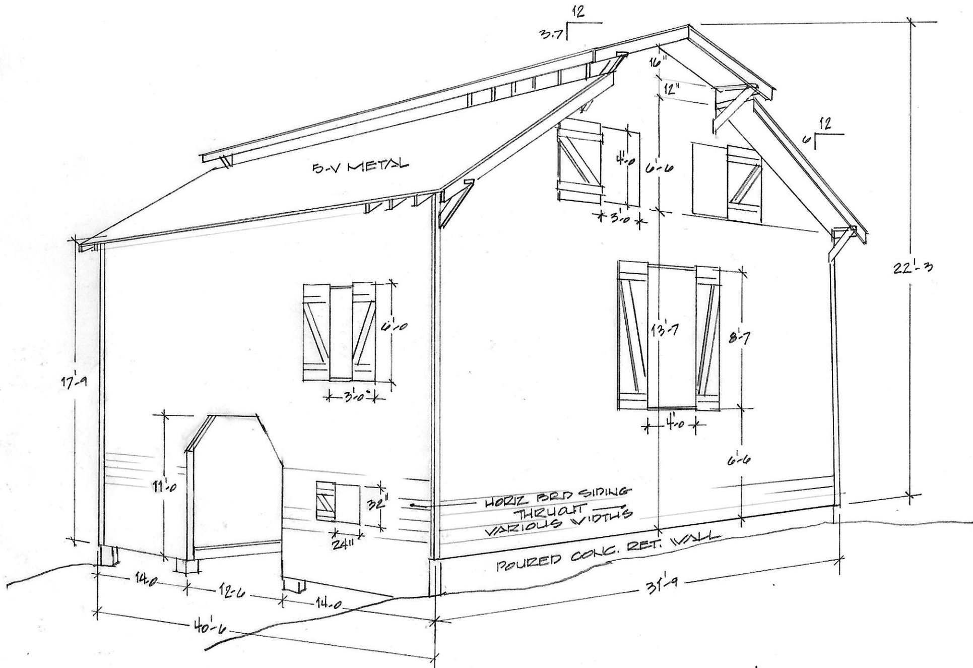
WOODS AMMONS BURLEY BARN #2 3/4 VIEW NO SCALE
