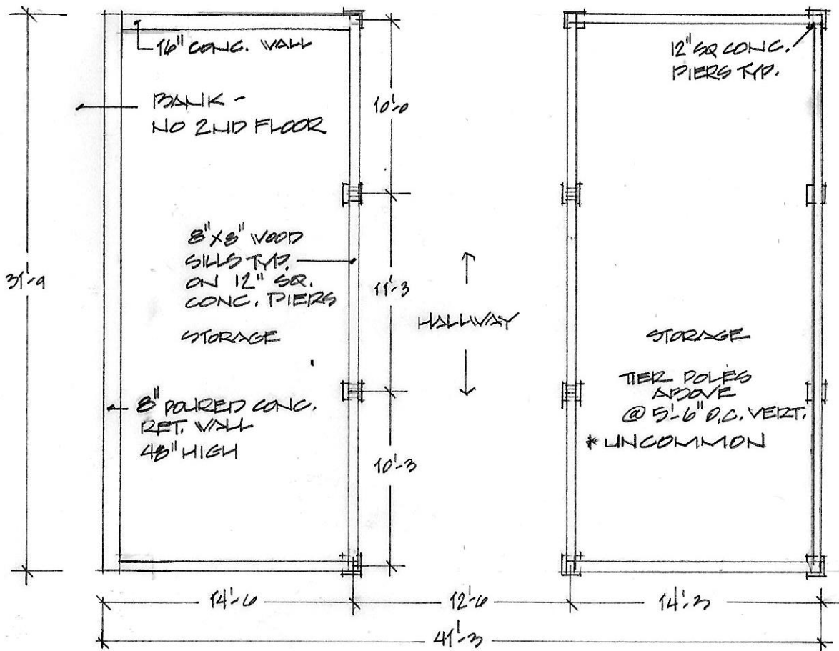
WOODS AMMONS BURLEY BARN #2 FLOOR PLAN - NO LOFT LEVEL \frac{1}{8}'' = 1'-0''
