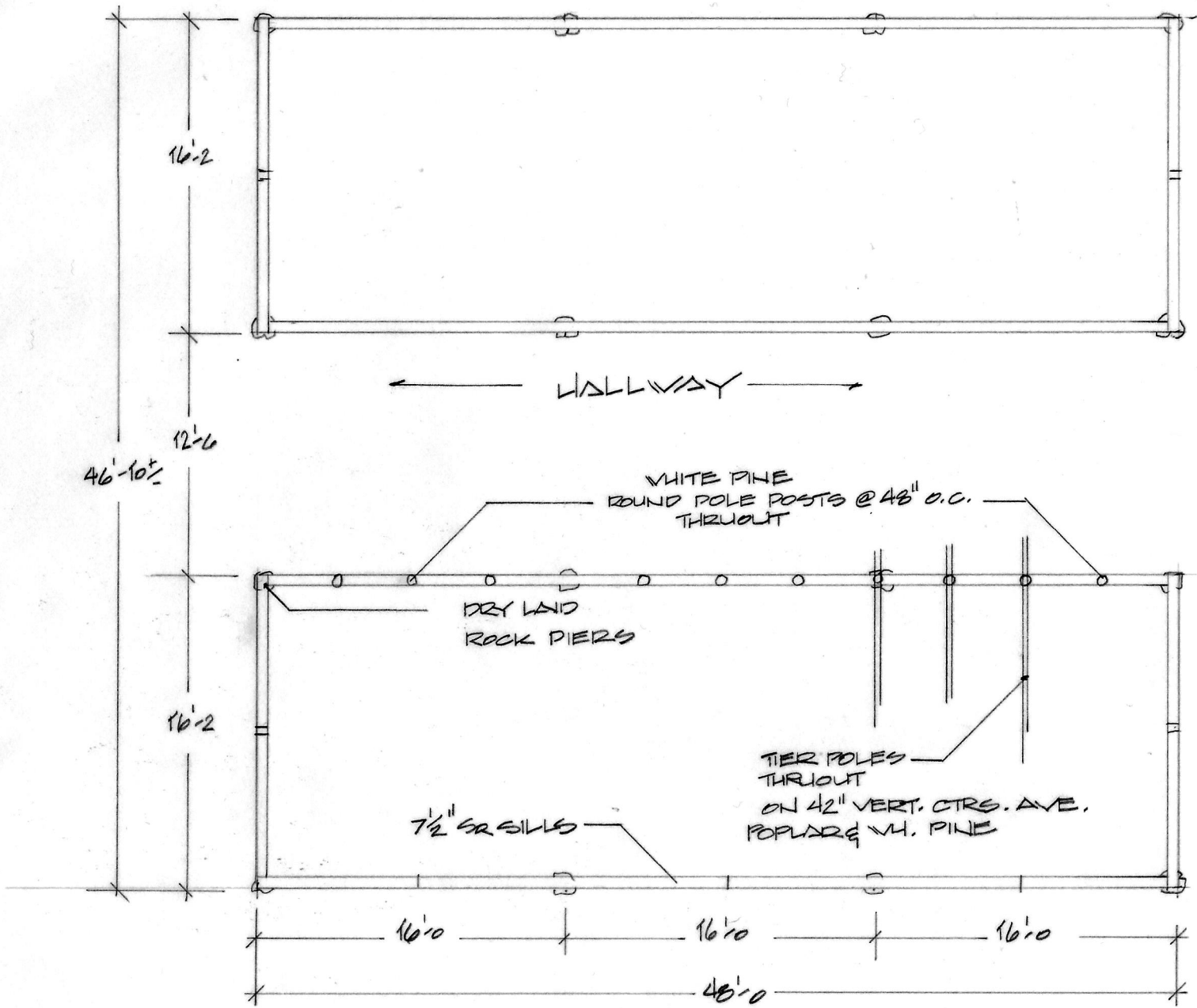
FLOOR PLAN SAMUEL MOORE-BURLEY
