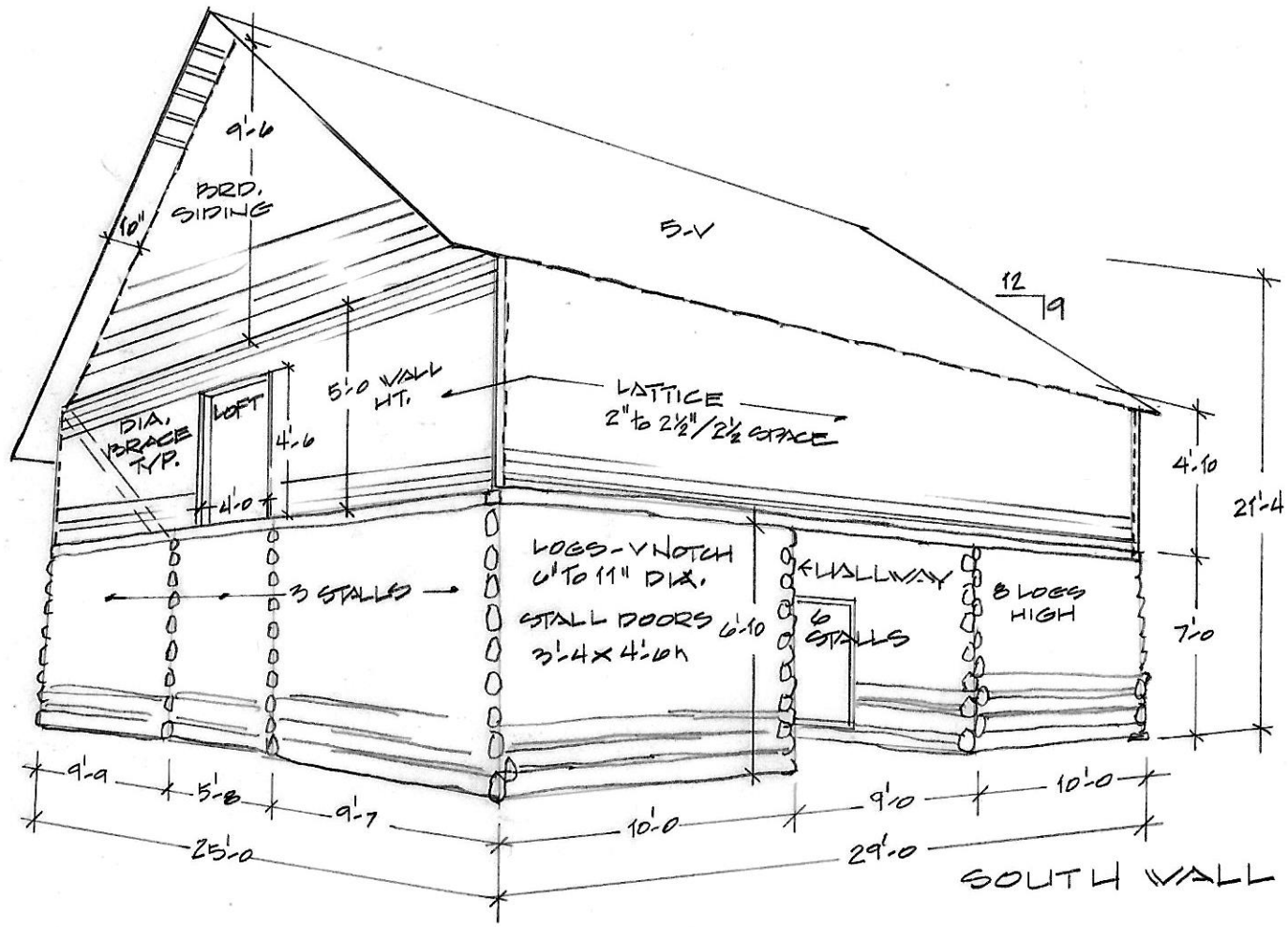
3/4 VIEW NO SCALE JIM PHILLIPS LIVESTOCK BARN
