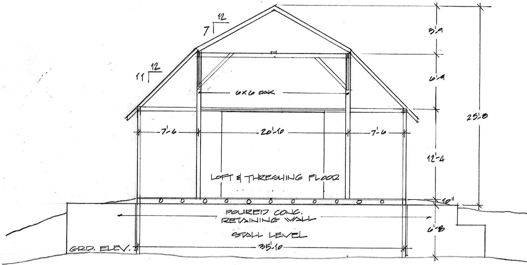
SECTION/ELEVATION \frac{1}{8}'' = 1'-0'' JETER ROBINSON LIVESTOCK BARN
