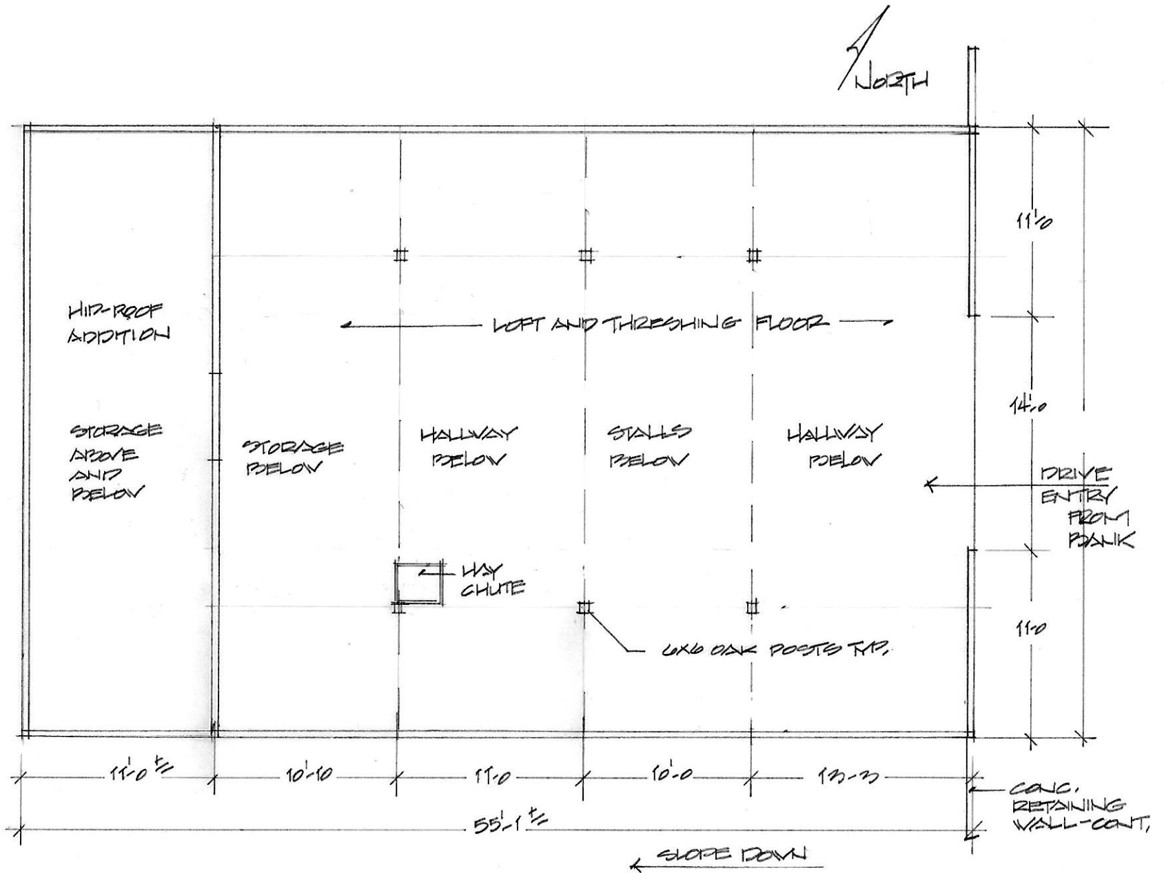
FLOOR PLAN - LOFT LEVEL JETER ROBINSON LIVESTOCK BARN
