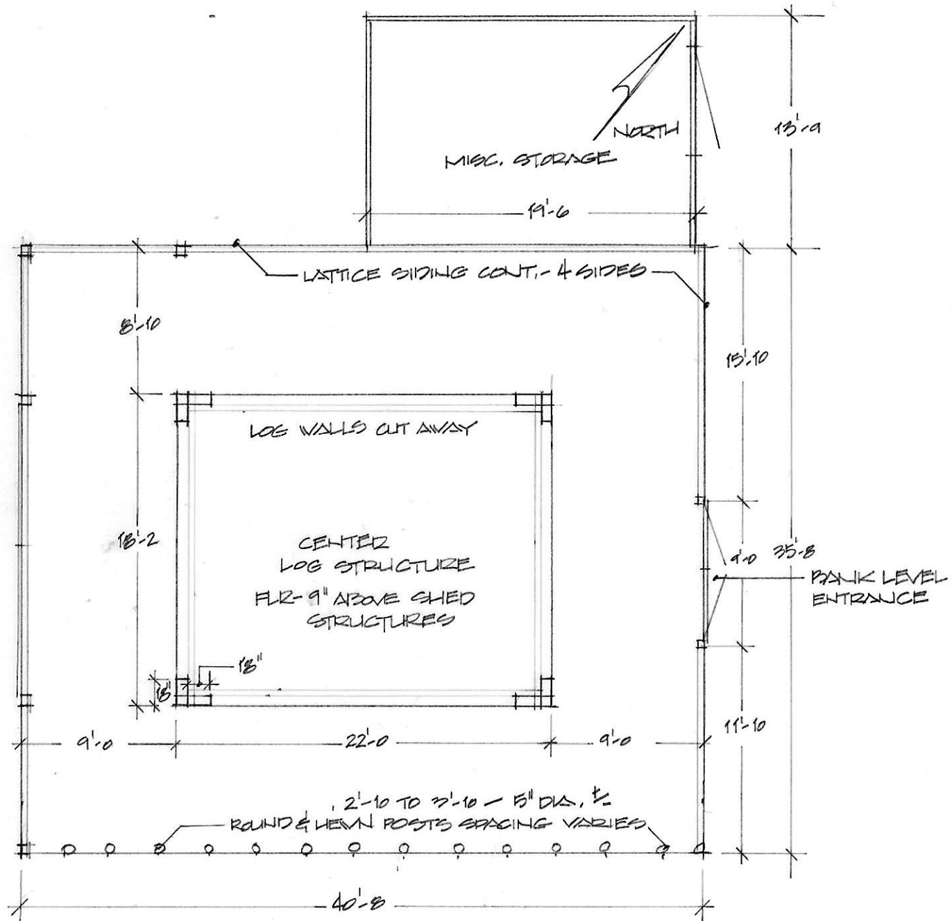
MAIN FLOOR - PLAN JACOB TILSON BARN
