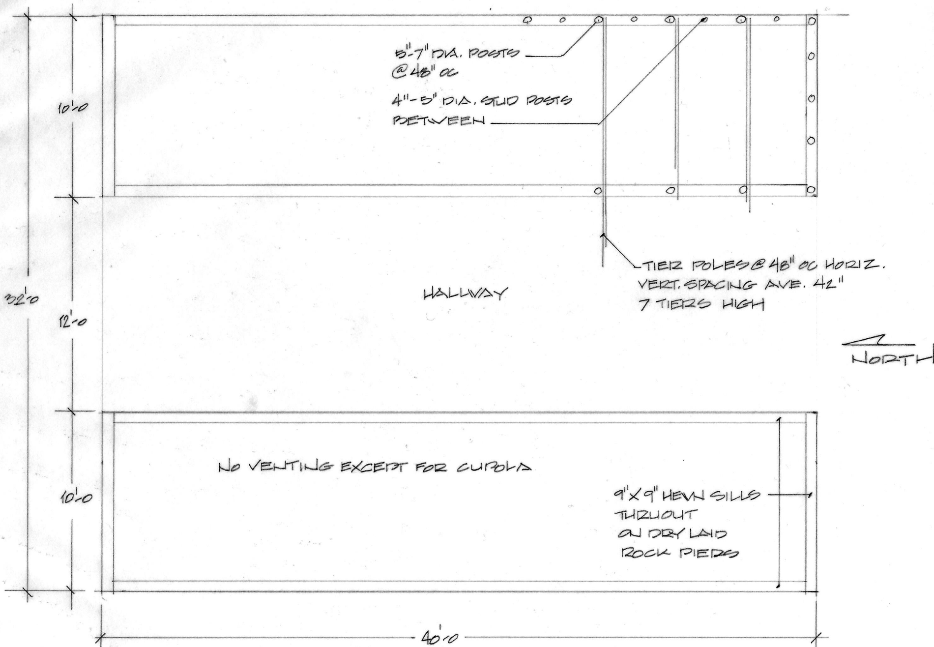
FLOOR PLAN \frac{3}{16}'' = 1'-0'' CURTIS BUCKNER BURLEY BARN
