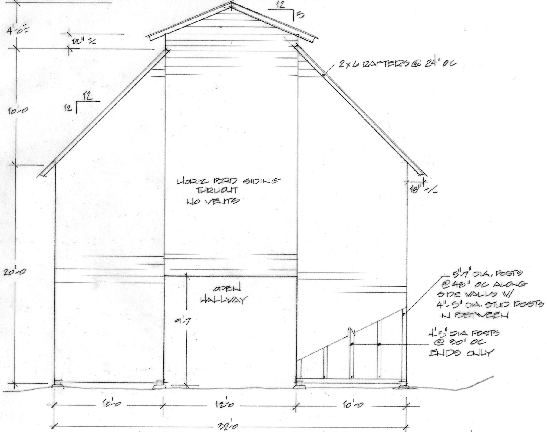
SOUTH ELEVATION 3/16" = 1'-0" CURTIS BUCKNER BURLEY TOBACCO
