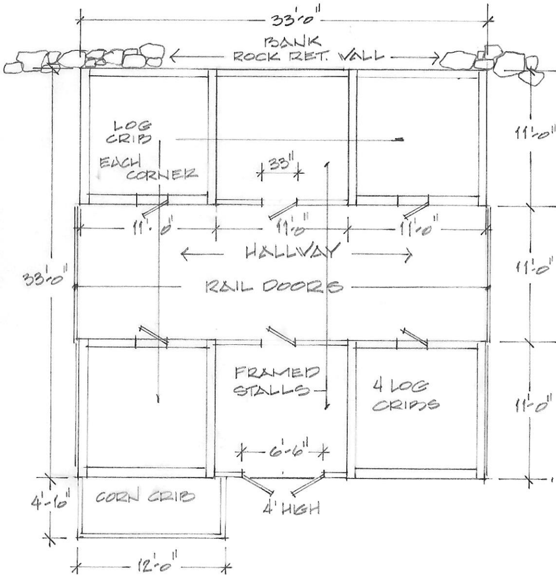
FLOOR PLAN - GROUND
