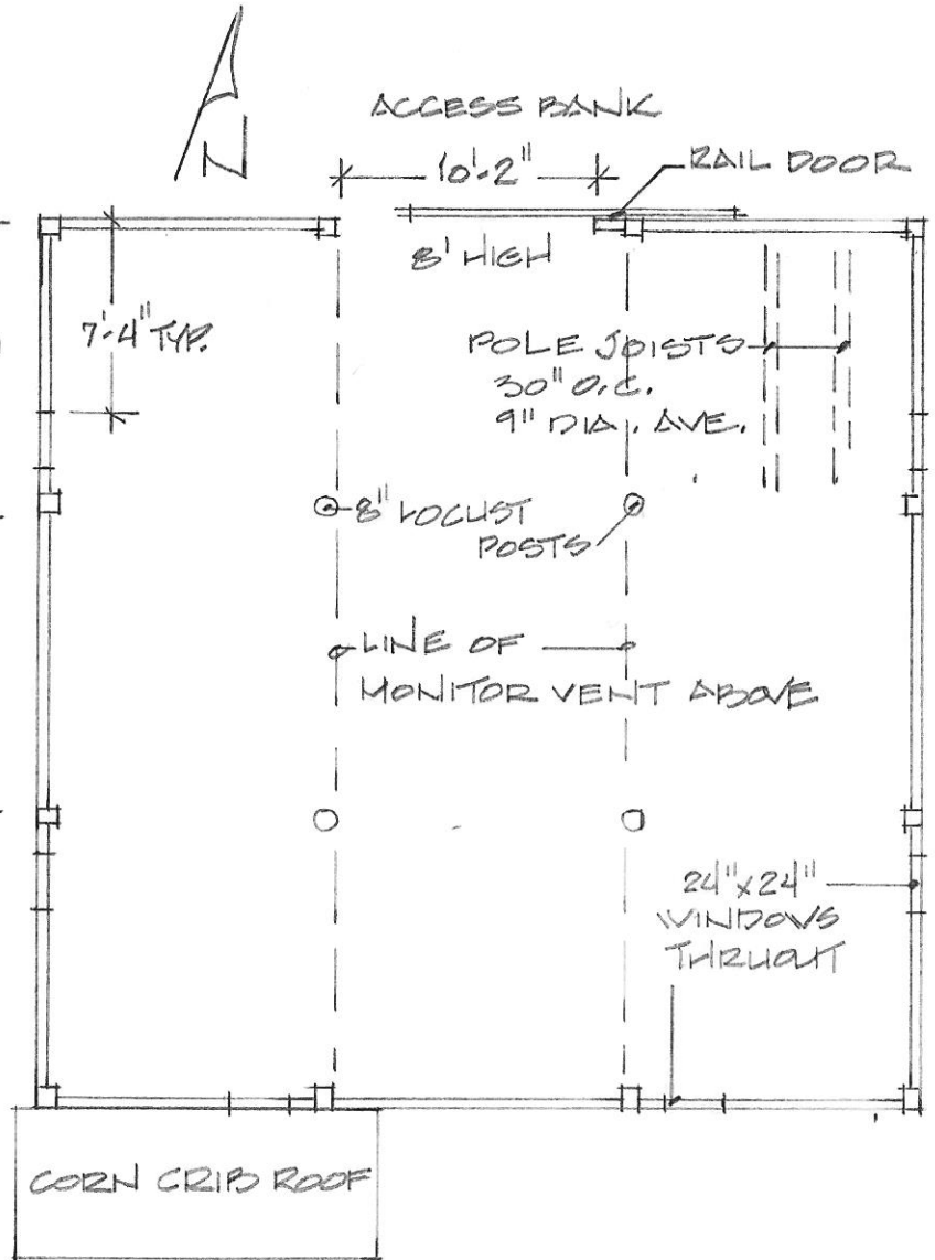
FLOOR PLAN - LOFT
