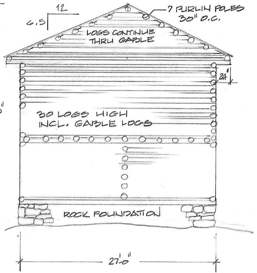
SOUTH ELEVATION
