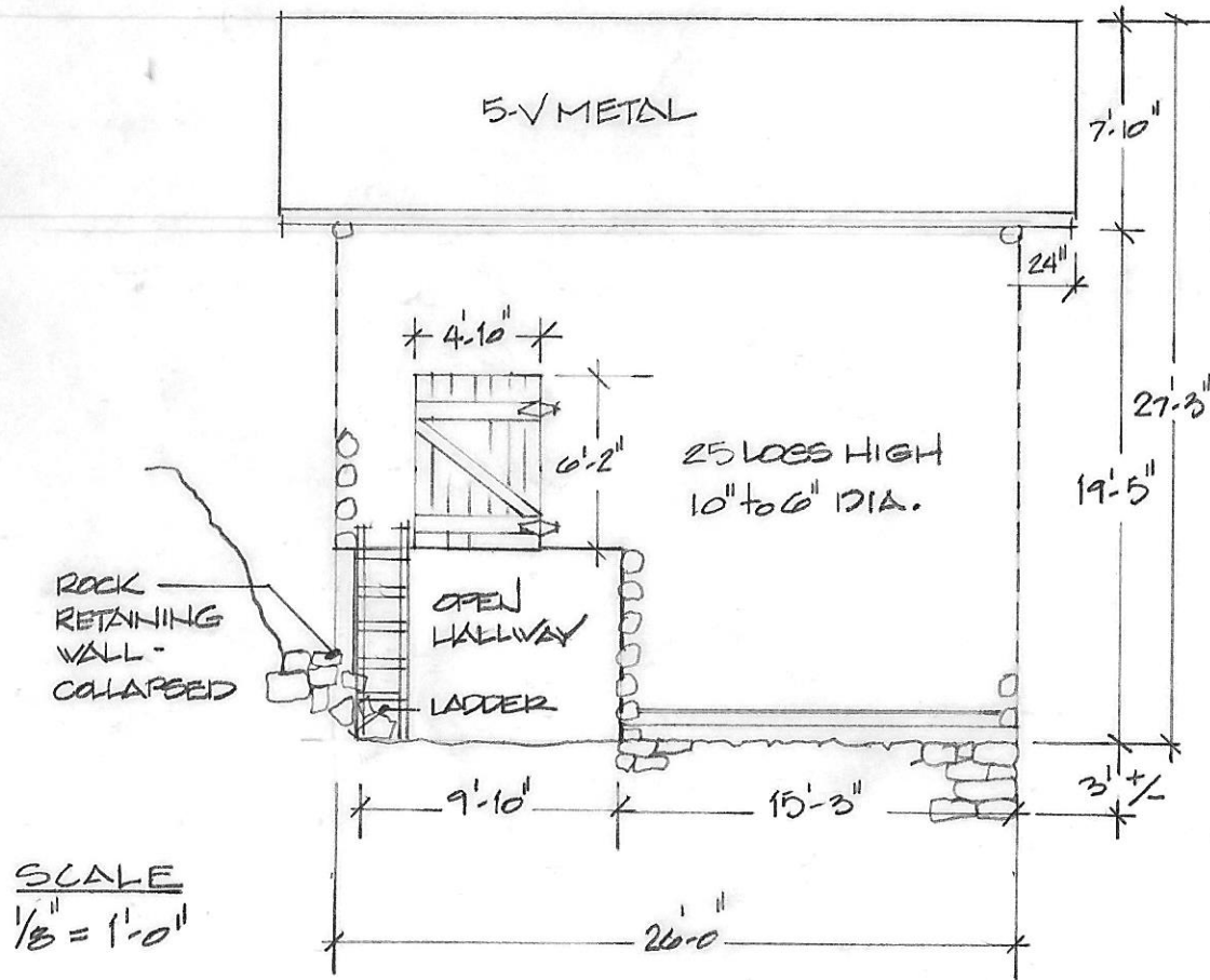
WEST ELEVATION
