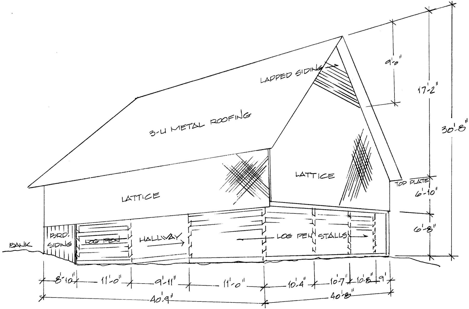
ISOMETRIC VIEW FROM SOUTH NO SCALE
